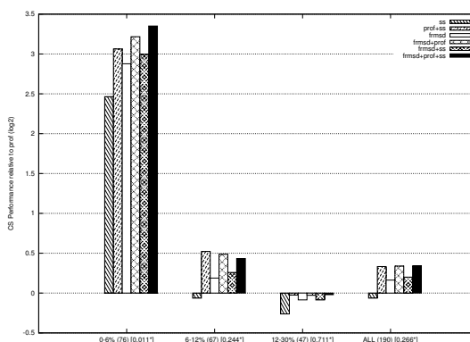
Fig. 3. Speedup using the Seeding and Sampling Alignment Procedure on the ce_ref dataset.
