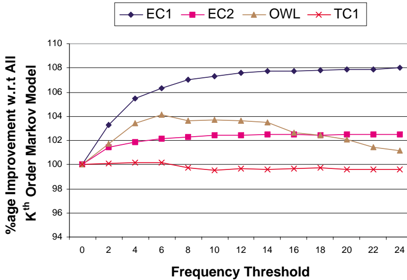
Figure 3: The accuracy obtained by SPMM for different values of \phi relative to that obtained by All- K^{\text{th}} -Order Markov model.
