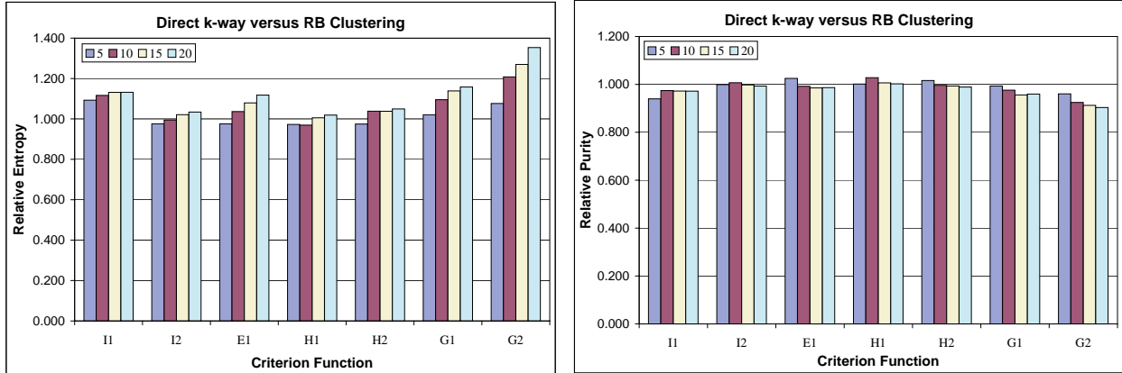
Figure 1: The relative performance of direct k -way clustering over that of repeated bisections (RB) averaged over the different datasets, for the entropy and purity measures.
