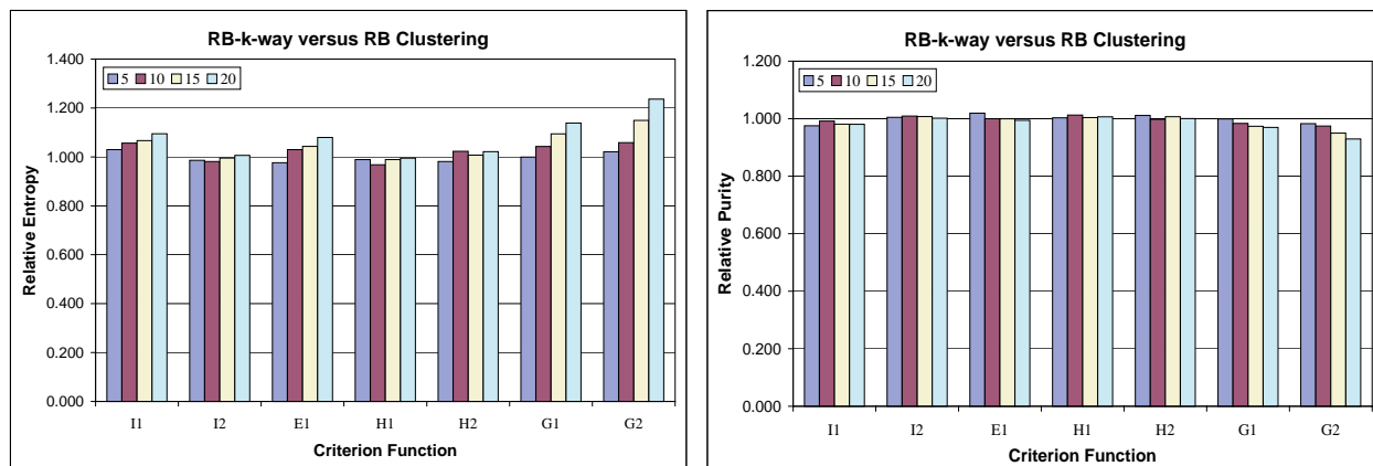
Figure 2: The relative performance of repeated bisections-based clustering followed by k -way refinement over that of repeated bisections alone. The results are averaged over the different datasets, for the entropy and purity measures.
